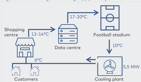
Fig 8.4: Tiered cooling and heating supply in Växjö
